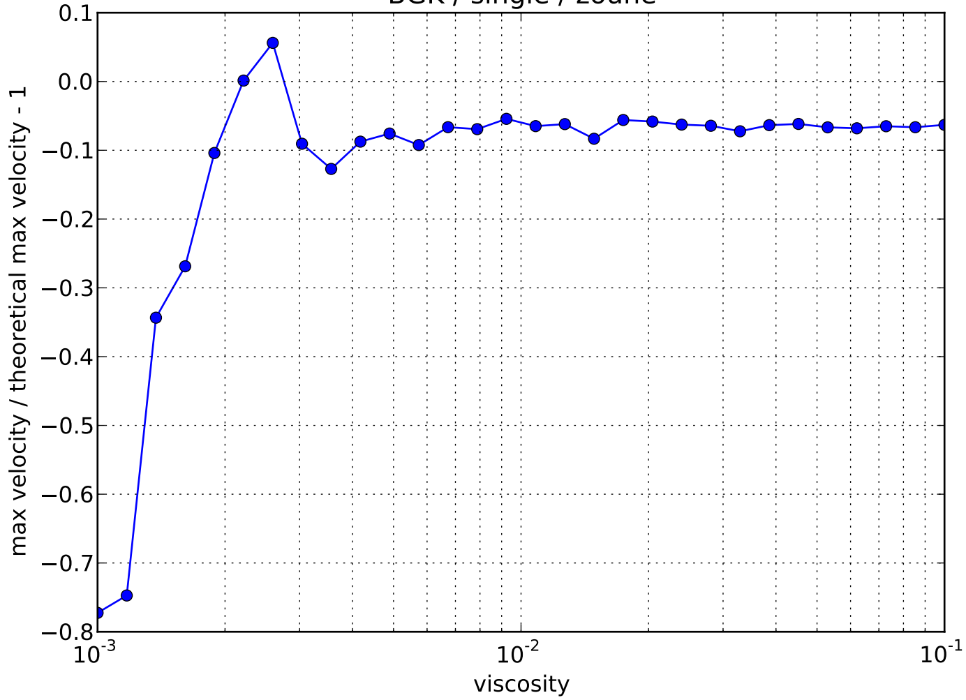
BGK / single / zouhe
