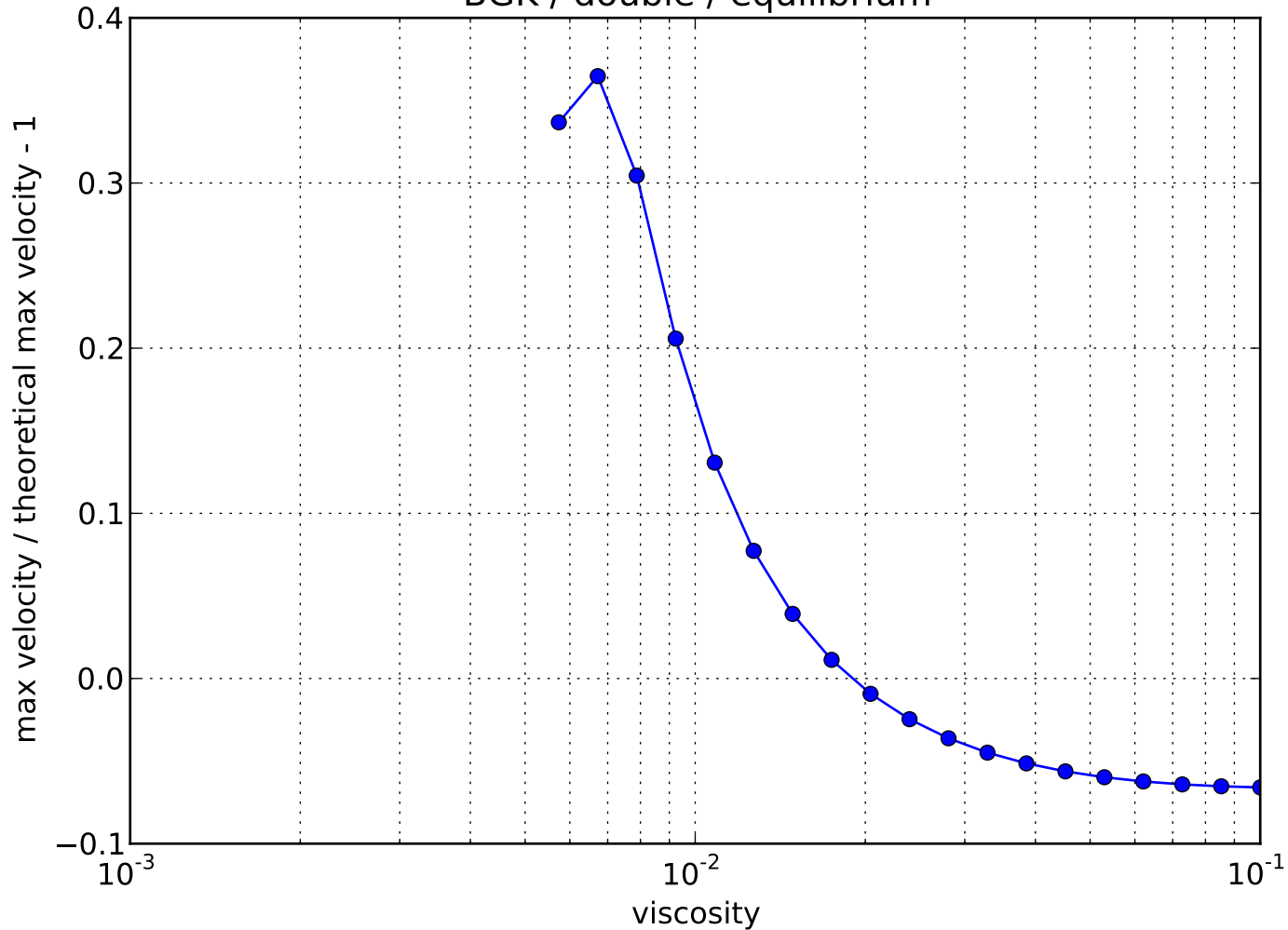
BGK / double / equilibrium
