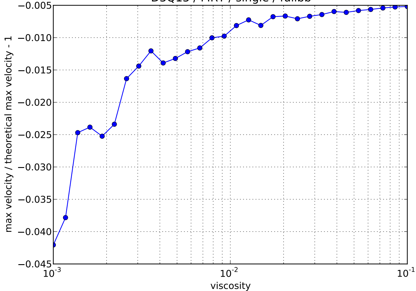
D3Q13 / MRT / single / fullbb
